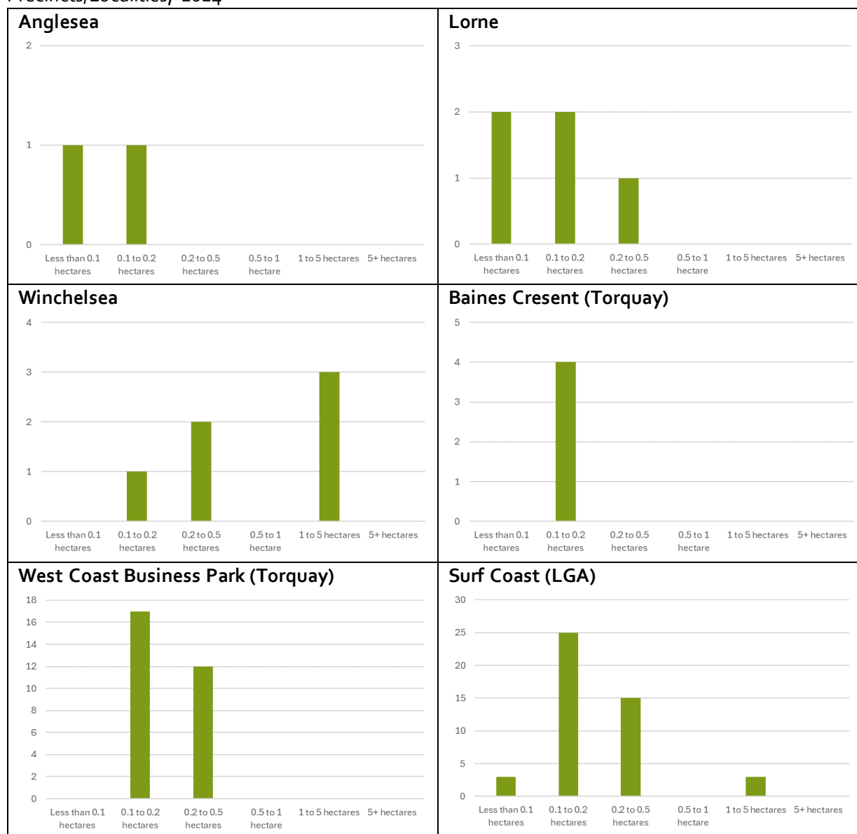
Graph 2: Number of Zoned Industrial Lots (Supply/Vacant) by Lot Size Range -Industrial Precincts/Localities, 2024
